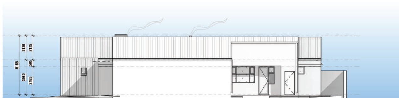
SOUTH ELEVATION
