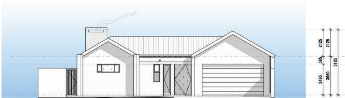
WEST ELEVATION
