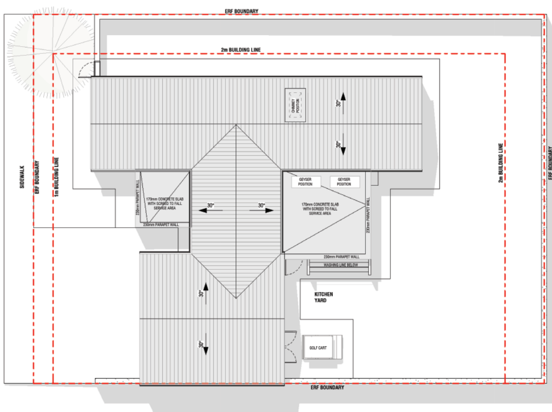
ROOF PLAN A2
