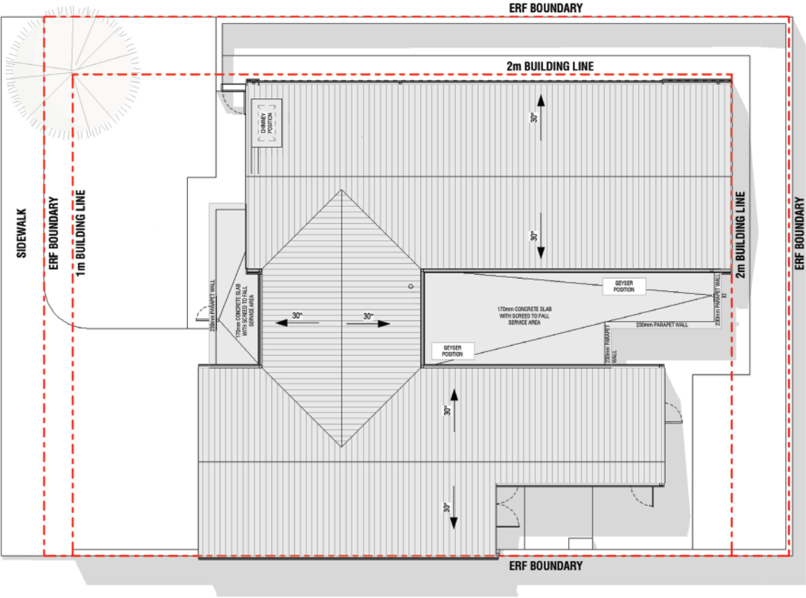
ROOF PLAN A3
