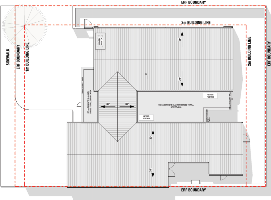
ROOF PLAN_A3
