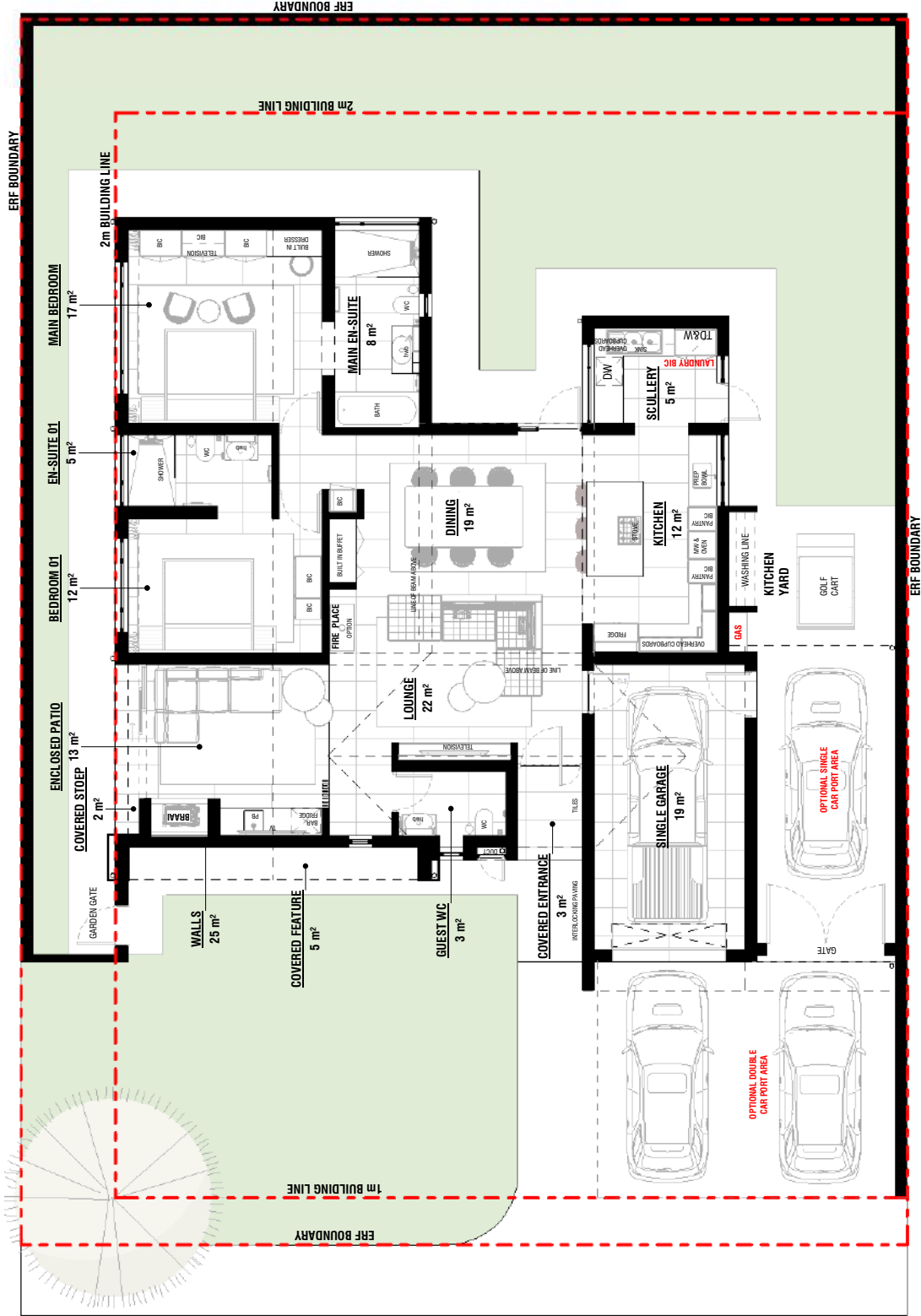
HOUSE TYPE A2 GROUND FLOOR AREA PLAN
