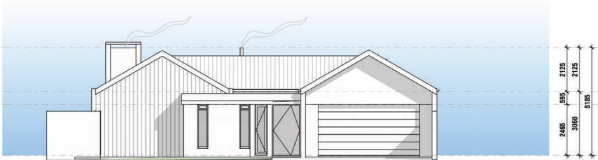
WEST ELEVATION
