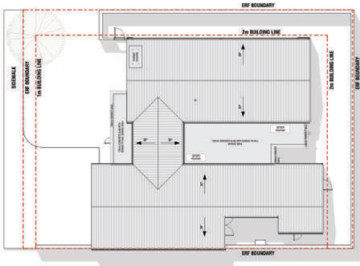
ROOF PLAN_A3
