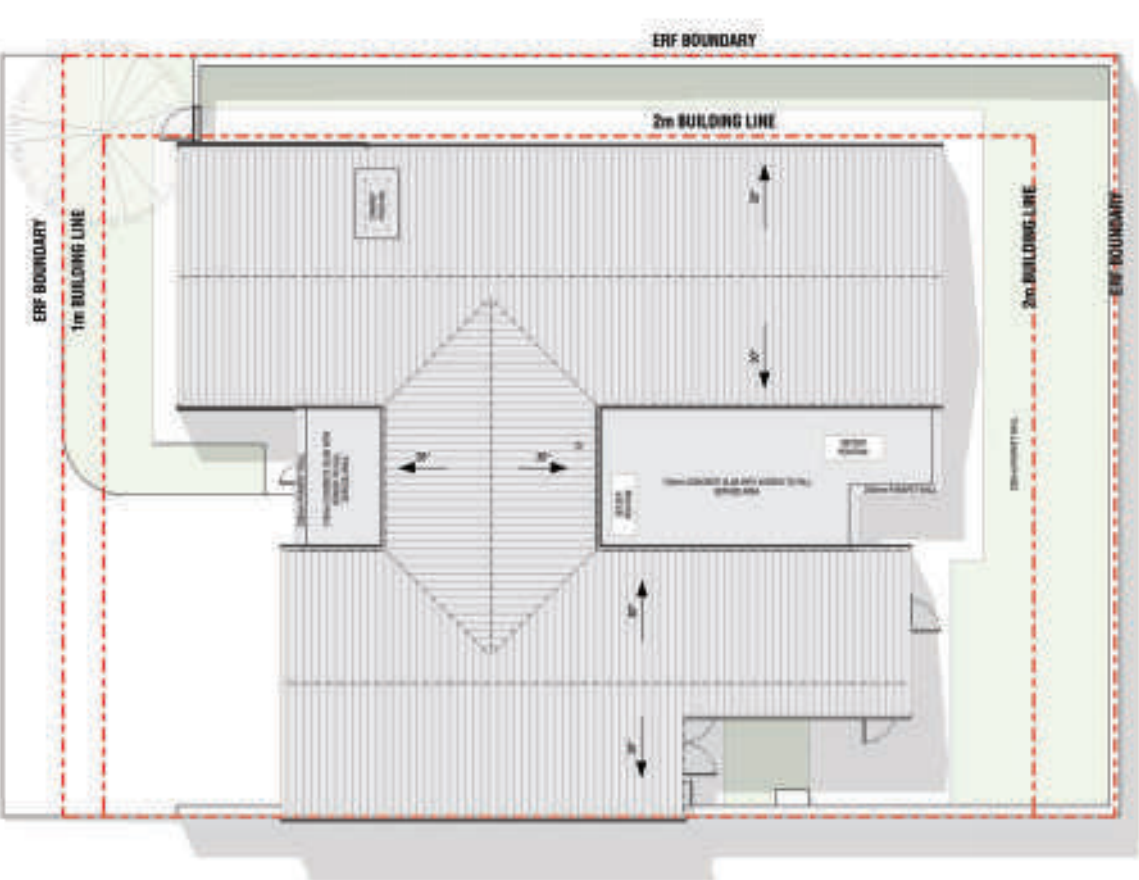
COVERAGE DIAGRAM SCALE: 1 : 500
