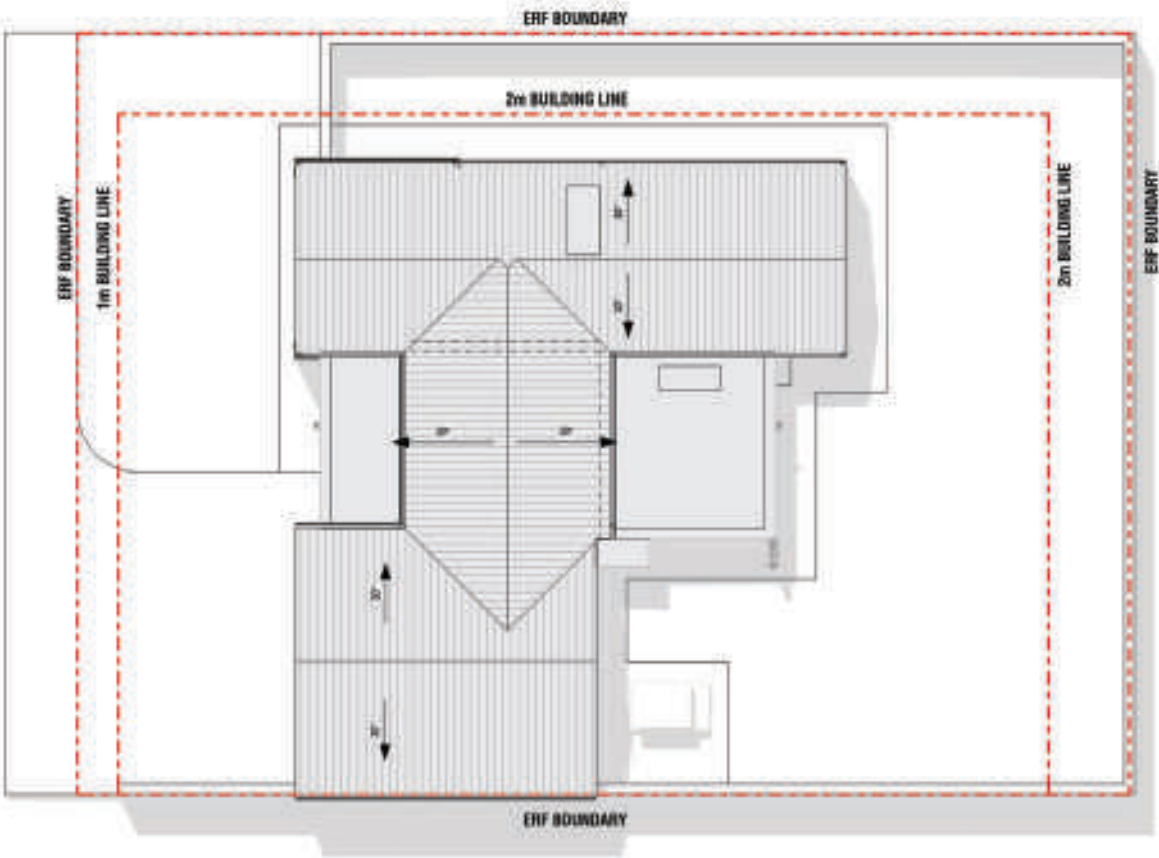
COVERAGE DIAGRAM SCALE: 1 : 500
