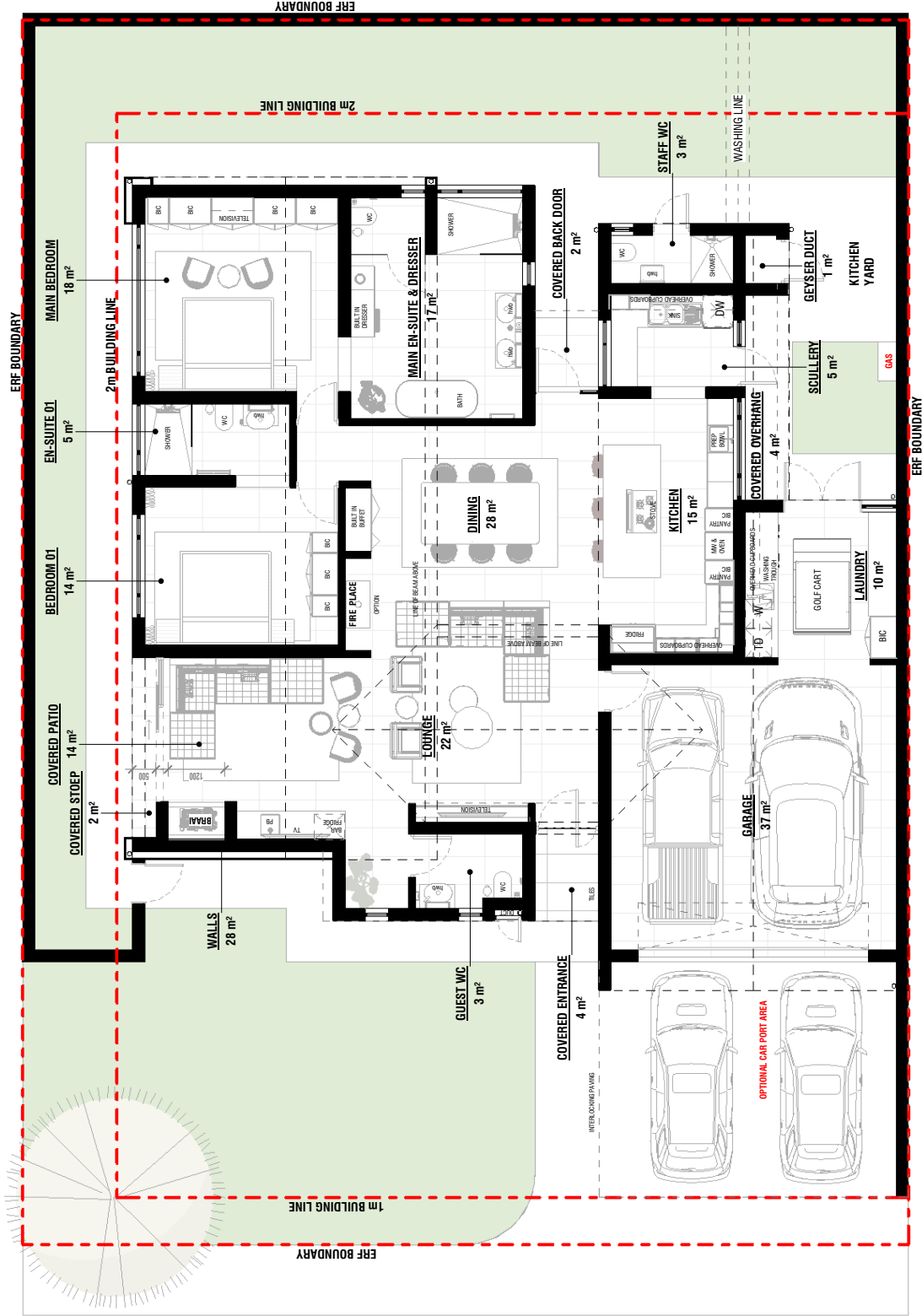
HOUSE TYPE A4 GROUND FLOOR AREA PLAN
