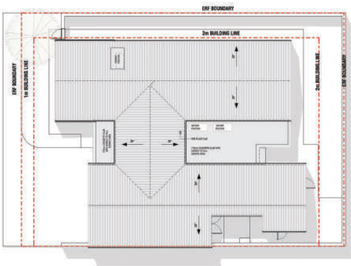
COVERAGE DIAGRAM SCALE: 1 : 500
